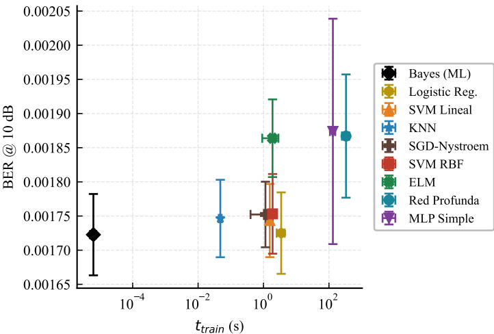
BER vs Training Cost Trade-off
